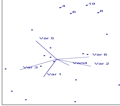
Figure 3: Visualisation of Wood dataset using xgobi . The outlier records are labelled 4, 6, 8 and 19.
